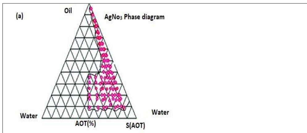
Figure 2: Pseudo-ternary phase diagram for systems of water in oil microemulsions that contain reducing agent (Palbociclib) and silver precursor (AgNO 3 ). D-Optimal mixture experimental technique
