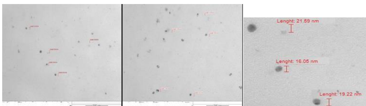
Figure 10: TEM images at lower and higher magnification of 12000 x and sizedistribution histogram of AgNPs loaded ME
