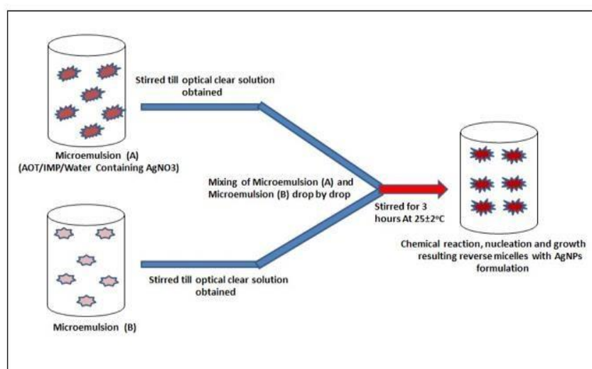
Figure 1: Diagrammatic representation of AgNPs synthesis using water-in-oil microemulsion
