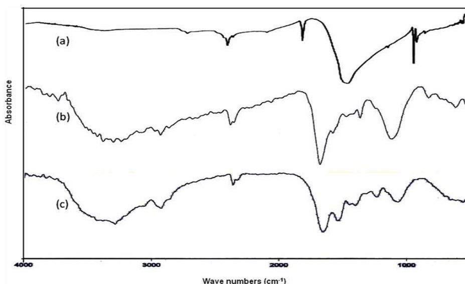
Figure 12: FTIR spectrum recorded by making KBr disc of (a) Palbociclib standard (b) Excipients mixture and synthesized (c) AgNPs loaded Microemulsion
