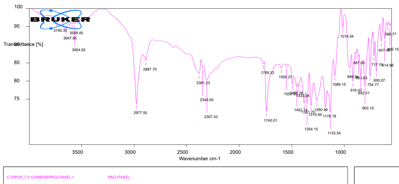
Figure: IR spectrum of Paclitaxel
