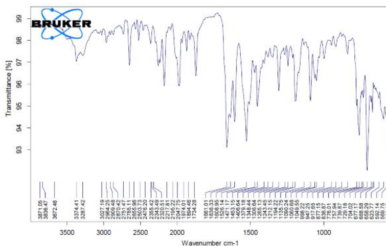
Figure 4: FT-IR Spectrum of Optimised Formulation (F2)
