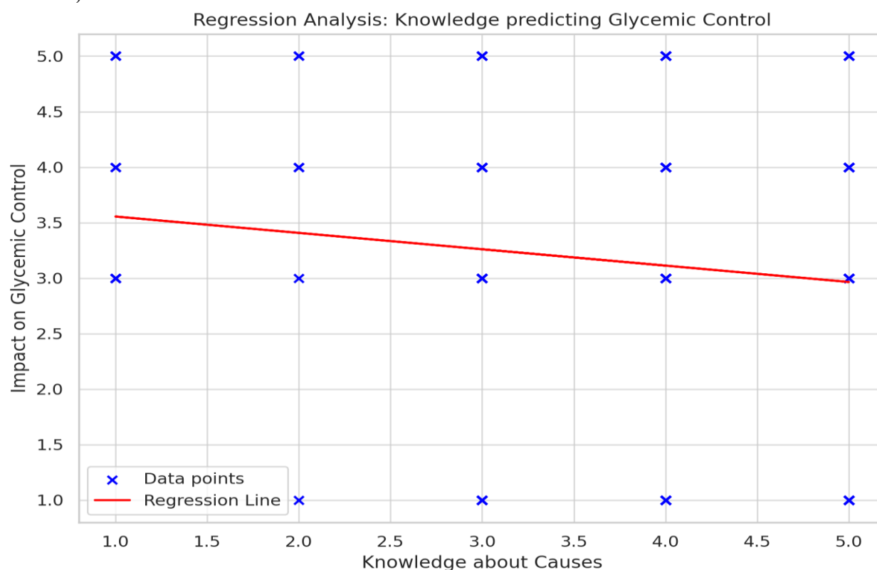
Figure 6: Regression Analysis
