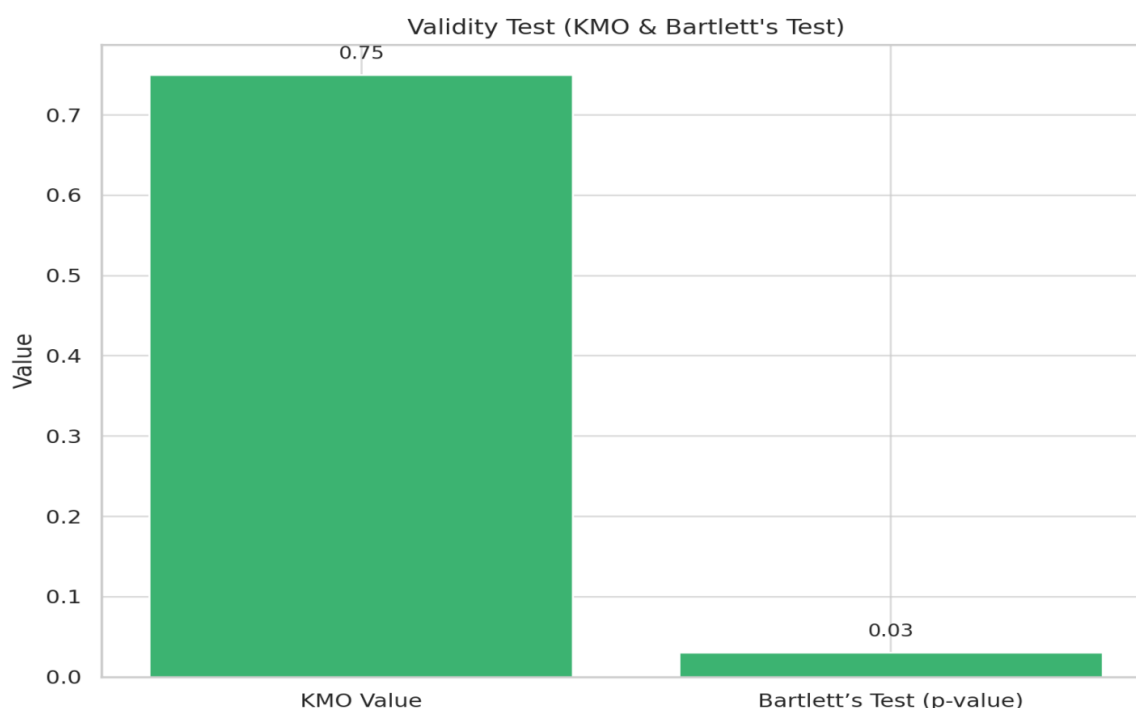
Figure 3: Validity Test (KMO & Bartlett's Test)
